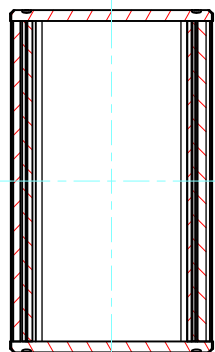
C-C (1:1.5)
